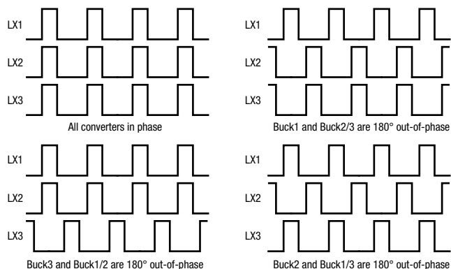
Figure 38. Out-of-Phase Operation
