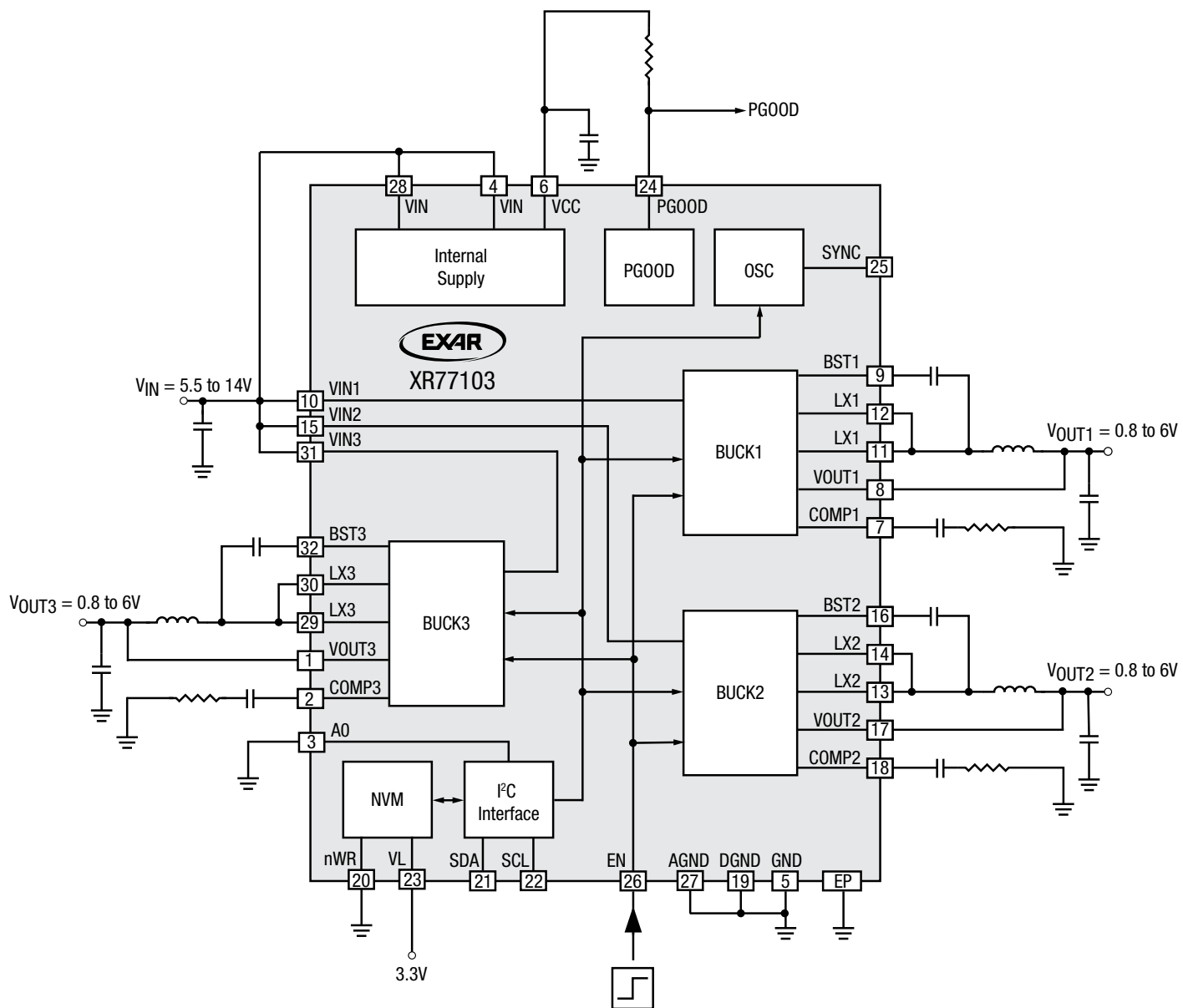
Figure 1. Typical Application
