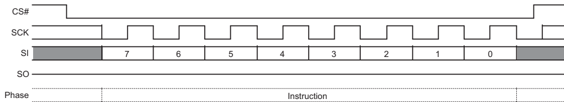
Figure 61. Write Enable (WREN) Command Sequence
