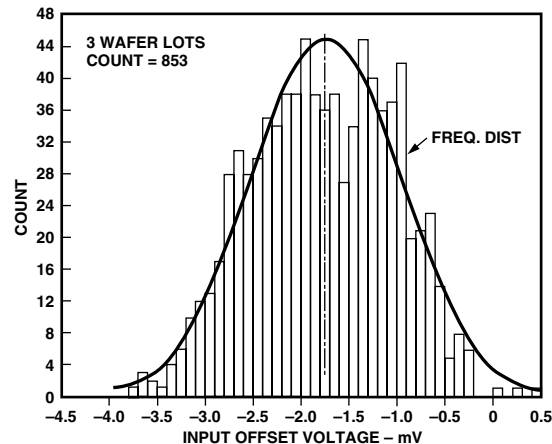
TPC 54. AD8037 Input Offset Voltage Distribution
