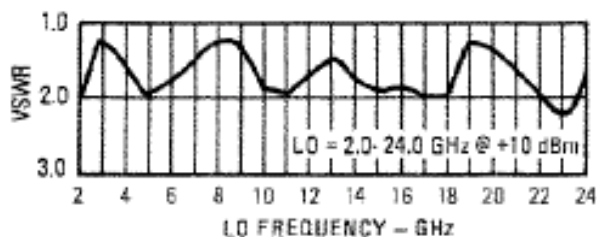
L-Port VSWR
