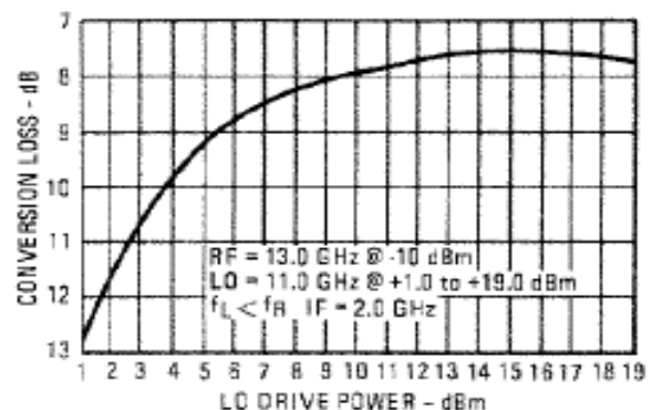
Drive Level
