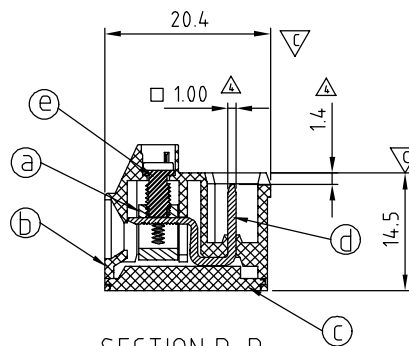
SECTION P-P
