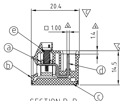
SECTION P-P
