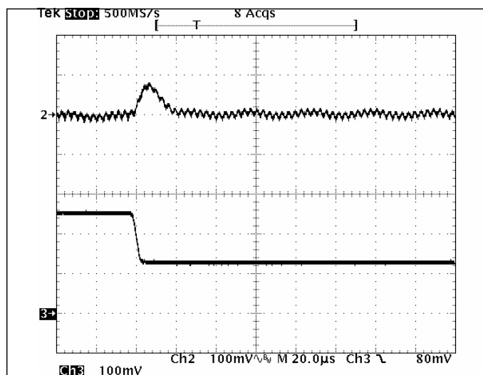
Fig 1.5V-7: Output voltage response for V_{out}=1.5V to negative load current step change from 5A to 2.5A with slew rate of -5A/\mu s at V_{in}=12V . C_o=47\mu F \times 2 ceramic. Top trace: output voltage (100mV/div.) Bottom trace: load current (2A/div.) Time scale: 20\mu s /div.
