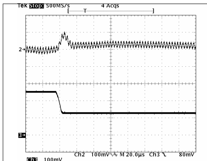
Fig 5.0V-7: Output voltage response for V_{out}=5.0V to negative load current step change from 5A to 2.5A with slew rate of -5A/\mu s at V_{in}=12V . C_o=47\mu F \times 2 ceramic. Top trace: output voltage (100mV/div.) Bottom trace: load current (2A/div.) Time scale: 20\mu s /div.
