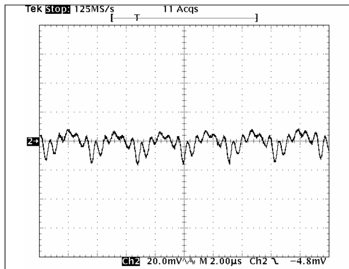
Fig 1.2V-5: Output voltage ripple (20mV/div.) for V_{out}=1.2V at full rated load current into a resistive load with external capacitance 47\mu F \times 2 ceramic + 1\mu F ceramic at V_{in}=12V . Time scale: 2\mu s /div.
