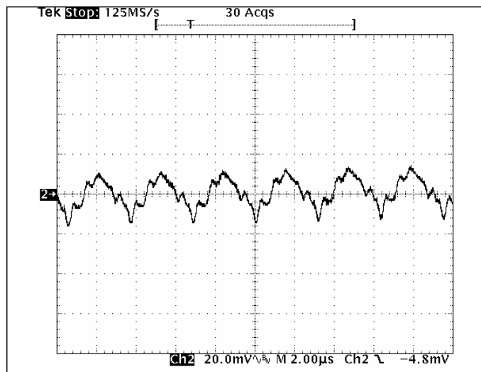
Fig 2.0V-5: Output voltage ripple (20mV/div.) for V_{out}=2.0V at full rated load current into a resistive load with external capacitance 47\mu F \times 2 ceramic + 1\mu F ceramic at V_{in}=12V . Time scale: 2\mu s /div.
