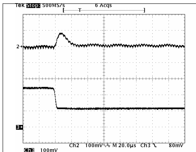
Fig 1.0V-7: Output voltage response for V_{out}=1.0V to negative load current step change from 5A to 2.5A with slew rate of -5A/\mu s at V_{in}=12V . C_o=47\mu F \times 2 ceramic. Top trace: output voltage (100mV/div.) Bottom trace: load current (2A/div.) Time scale: 20\mu s /div.
