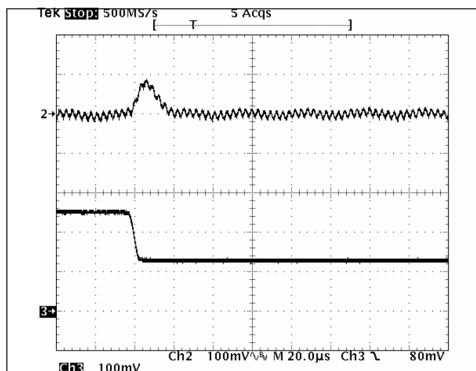
Fig 2.0V-7: Output voltage response for V_{out}=2.0V to negative load current step change from 5A to 2.5A with slew rate of -5A/\mu s at V_{in}=12V . C_o=47\mu F \times 2 ceramic. Top trace: output voltage (100mV/div.) Bottom trace: load current (2A/div.) Time scale: 20\mu s /div.
