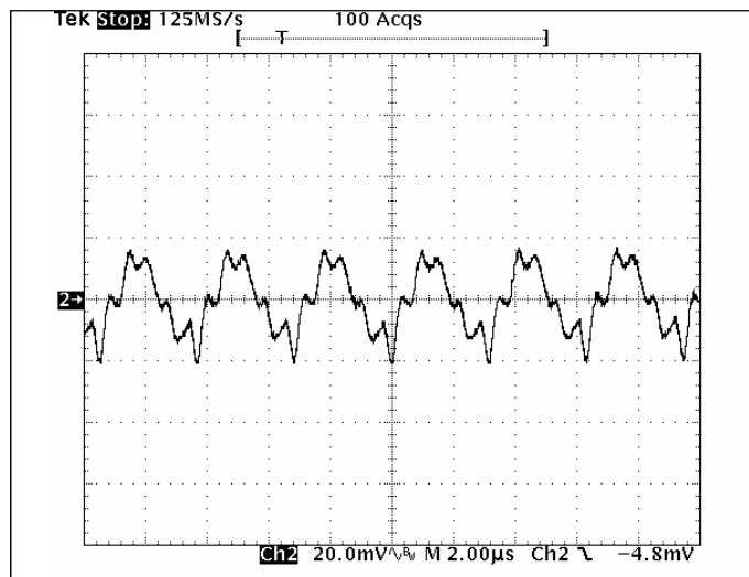
Fig 3.3V-5: Output voltage ripple (20mV/div.) for V_{out}=3.3V at full rated load current into a resistive load with external capacitance 47\mu F \times 2 ceramic + 1\mu F ceramic at V_{in}=12V . Time scale: 2\mu s /div.
