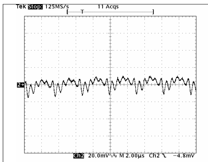
Fig 1.0V-5: Output voltage ripple (20mV/div.) for V_{out}=1.0V at full rated load current into a resistive load with external capacitance 47\mu F \times 2 ceramic + 1\mu F ceramic at V_{in}=12V . Time scale: 2\mu s /div.
