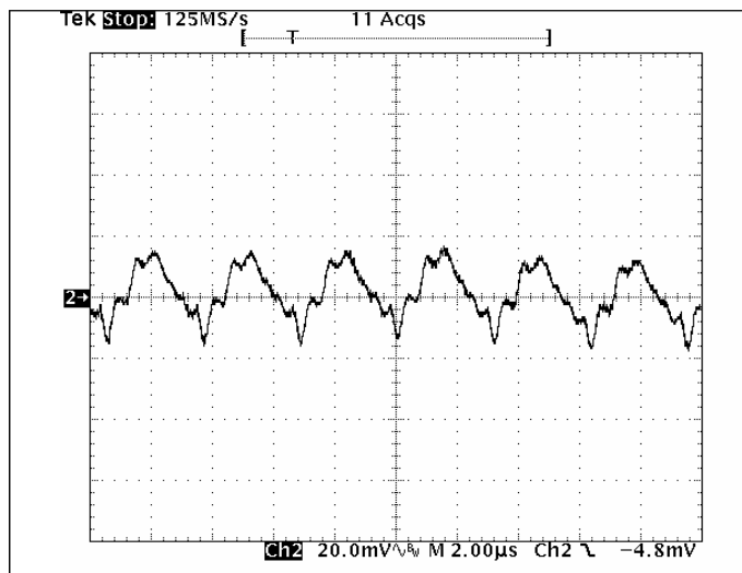
Fig 2.5V-5: Output voltage ripple (20mV/div.) for V_{out}=2.5V at full rated load current into a resistive load with external capacitance 47\mu F \times 2 ceramic + 1\mu F ceramic at V_{in}=12V . Time scale: 2\mu s /div.
