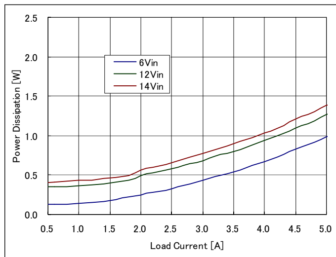
Fig 2.5V-3: Power Loss vs. load current and input voltage for V_{out}=2.5V . Airflow rate = 200LFM (1m/s) and T_a=25^{\circ}C .
