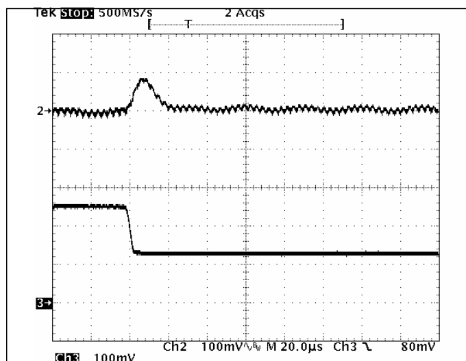
Fig 1.2V-7: Output voltage response for V_{out}=1.2V to negative load current step change from 5A to 2.5A with slew rate of -5A/\mu s at V_{in}=12V . C_o=47\mu F \times 2 ceramic. Top trace: output voltage (100mV/div.) Bottom trace: load current (2A/div.) Time scale: 20\mu s /div.
