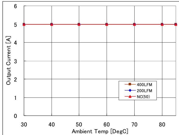
Fig 1.8V-1: Available load current vs. ambient temperature and airflow rates for V_{out}=1.8V with V_{in}=12V . Maximum component temperature \leq 120^{\circ}C .
