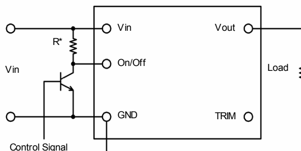
Fig. A: Circuit configuration for remote ON/OFF
