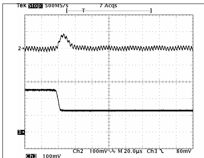
Fig 2.5V-7: Output voltage response for V_{out}=2.5V to negative load current step change from 5A to 2.5A with slew rate of -5A/\mu s at V_{in}=12V . C_o=47\mu F \times 2 ceramic. Top trace: output voltage (100mV/div.) Bottom trace: load current (2A/div.) Time scale: 20\mu s /div.
