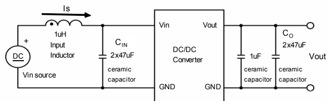
Fig. D: Test setup for measuring output voltage ripple
