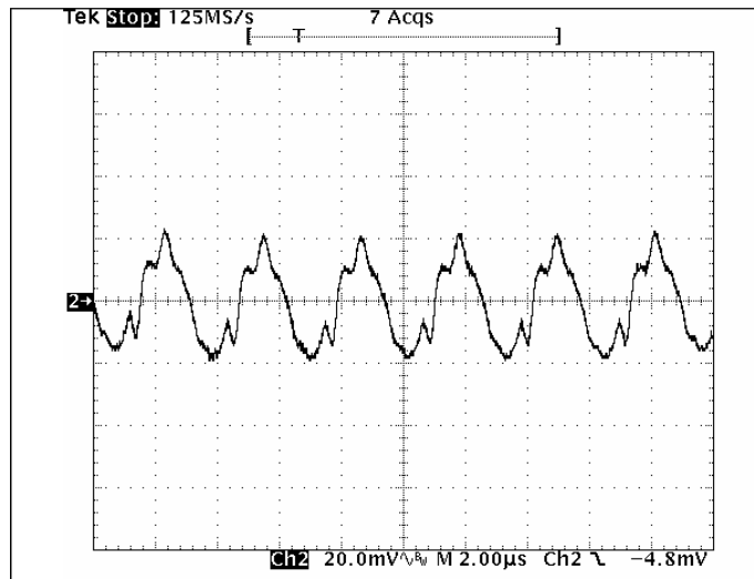
Fig 5.0V-5: Output voltage ripple (20mV/div.) for V_{out}=5.0V at full rated load current into a resistive load with external capacitance 47\mu F \times 2 ceramic + 1\mu F ceramic at V_{in}=12V . Time scale: 2\mu s /div.
