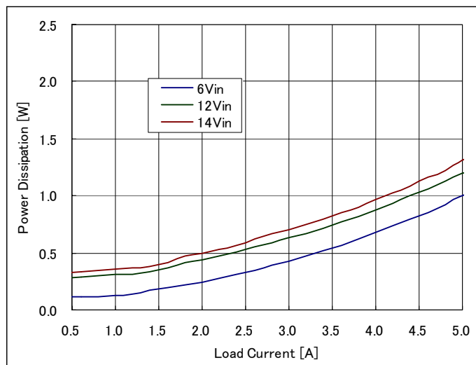
Fig 2.0V-3: Power Loss vs. load current and input voltage for V_{out}=2.0V . Airflow rate = 200LFM (1m/s) and T_a=25^{\circ}C .
