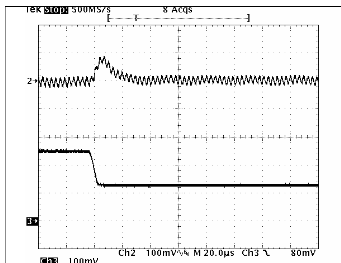
Fig 3.3V-7: Output voltage response for V_{out}=3.3V to negative load current step change from 5A to 2.5A with slew rate of -5A/\mu s at V_{in}=12V . C_o=47\mu F \times 2 ceramic. Top trace: output voltage (100mV/div.) Bottom trace: load current (2A/div.) Time scale: 20\mu s /div.
