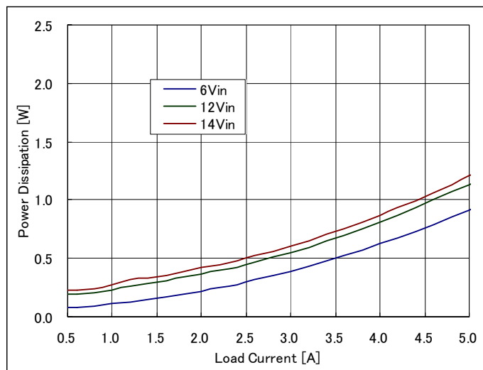
Fig 1.2V-3: Power Loss vs. load current and input voltage for V_{out}=1.2V . Airflow rate = 200LFM (1m/s) and T_a=25^{\circ}C .
