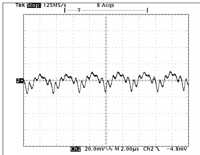
Fig 1.5V-5: Output voltage ripple (20mV/div.) for V_{out}=1.5V at full rated load current into a resistive load with external capacitance 47\mu F \times 2 ceramic + 1\mu F ceramic at V_{in}=12V . Time scale: 2\mu s /div.
