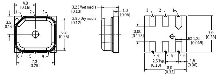
FIGURE 7. LEADLESS SMT PACKAGE DIMENSIONAL DRAWINGS (FOR REFERENCE ONLY: MM [IN].)
