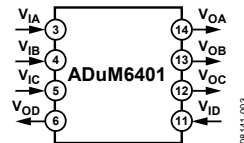
Figure 3. ADuM6401
