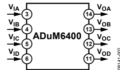
Figure 2. ADuM6400
