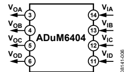
Figure 6. ADuM6404
