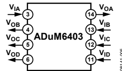
Figure 5. ADuM6403
