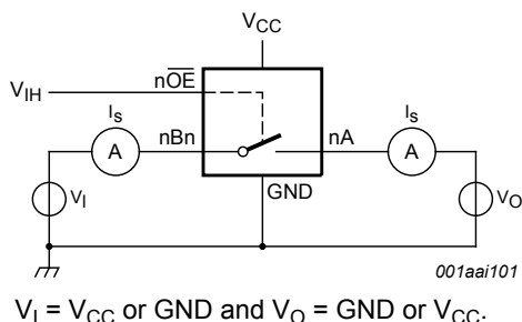
Fig. 5. Test circuit for measuring OFF-state leakage current (one switch)
