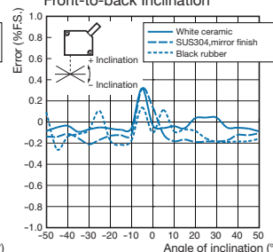
Front-to-back Inclination
