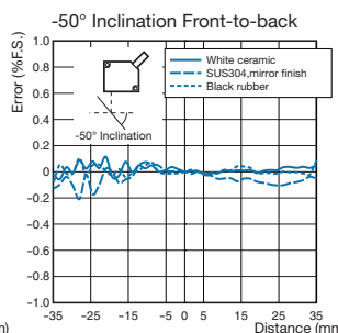
-50° Inclination Front-to-back
