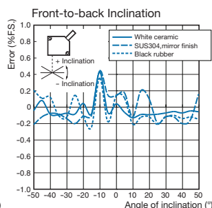
Front-to-back Inclination
