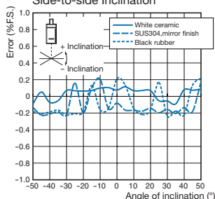
Side-to-side Inclination
