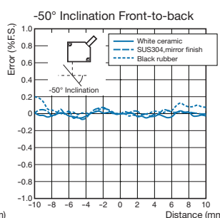
-50° Inclination Front-to-back
