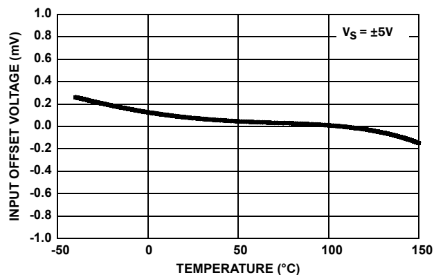
FIGURE 2. INPUT OFFSET VOLTAGE vs TEMPERATURE
