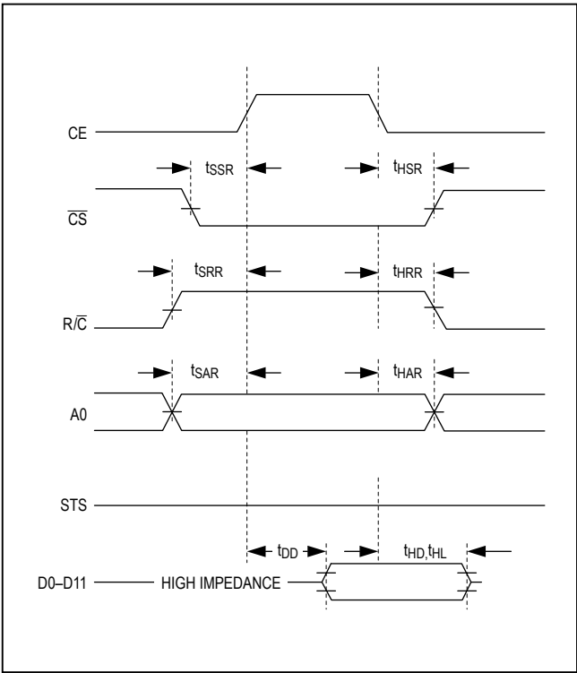
Figure 5. Read Timing
