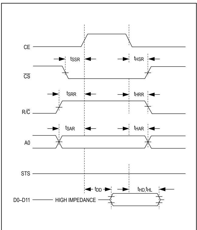
Figure 5. Read Timing
