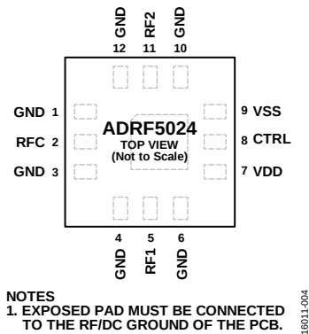
Figure 4. Pin Configuration (Top View)
