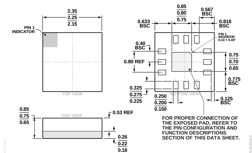
Figure 26. 12-Terminal Land Grid Array [LGA] 2.25 mm × 2.25 mm Body and 0.75 mm Package Height (CC-12-3) Dimensions shown in millimeters
