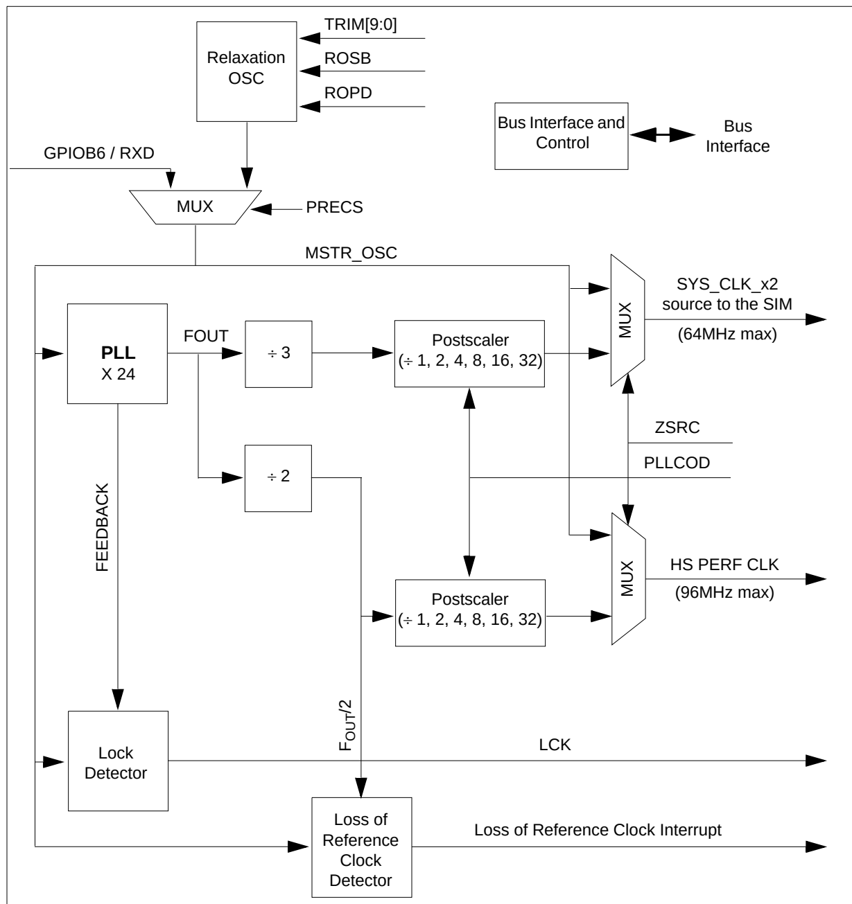
Figure 3-2 OCCS Block Diagram with Relaxation Oscillator
