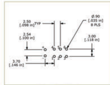
PC MOUNTING
