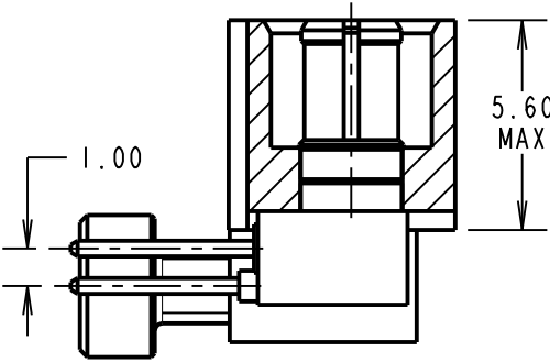
SECTION Z-Z
