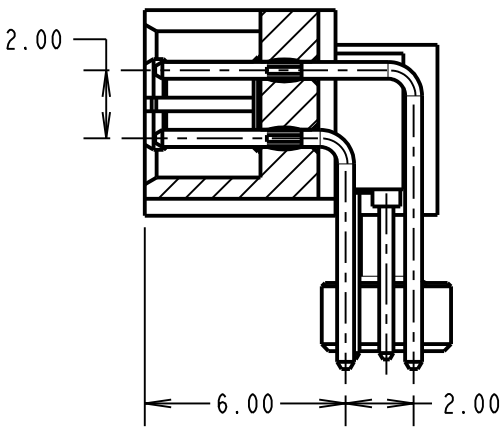
SECTION X-X
