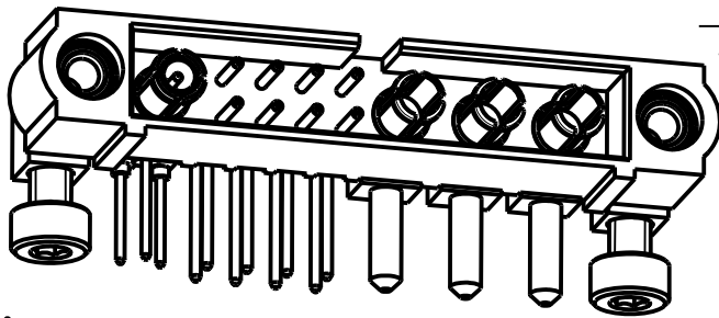
VIEW OF POWER CONTACT
