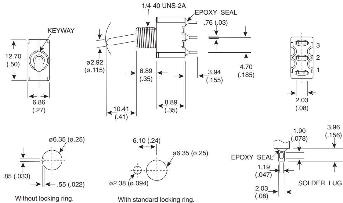
PANEL MOUNTING
