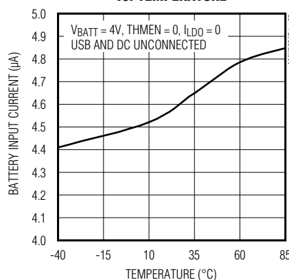
BATTERY INPUT CURRENT vs. TEMPERATURE
