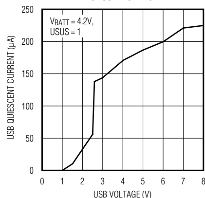
USB SUSPEND CURRENT vs. USB VOLTAGE
