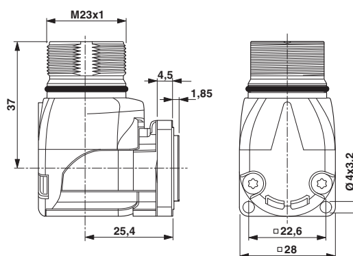
Dimensional drawing
