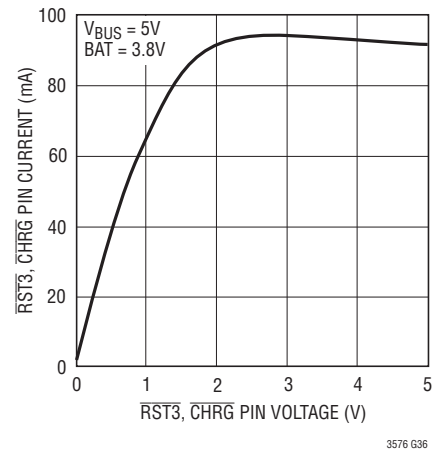
RST3, CHR3 Pin Current vs Voltage (Pull-Down State)
