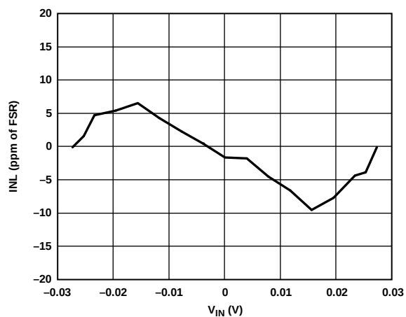
Figure 14. INL (Gain = 128)
