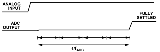
Figure 31. Sinc 4 Zero Latency Operation
