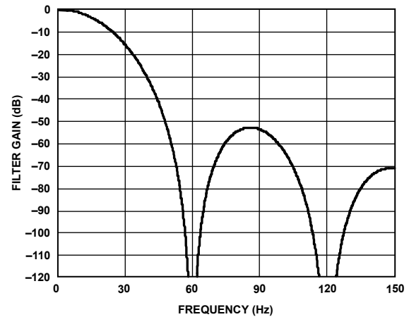
Figure 33. Sinc 4 Filter Response (FS[9:0] = 80)
