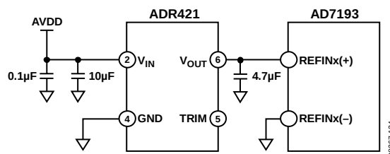
Figure 23. ADR421 to AD7193 Connections
