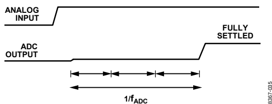
Figure 39. Sinc 3 Zero Latency Operation
