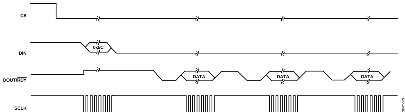
Figure 27. Continuous Read
