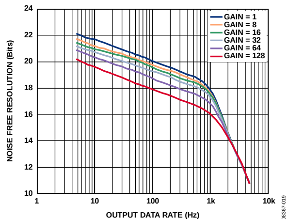
Figure 20. Noise Free Resolution ( \text{Sinc}^3 Filter, Chop Disabled, V_{\text{REF}} = 5 \text{ V} )
