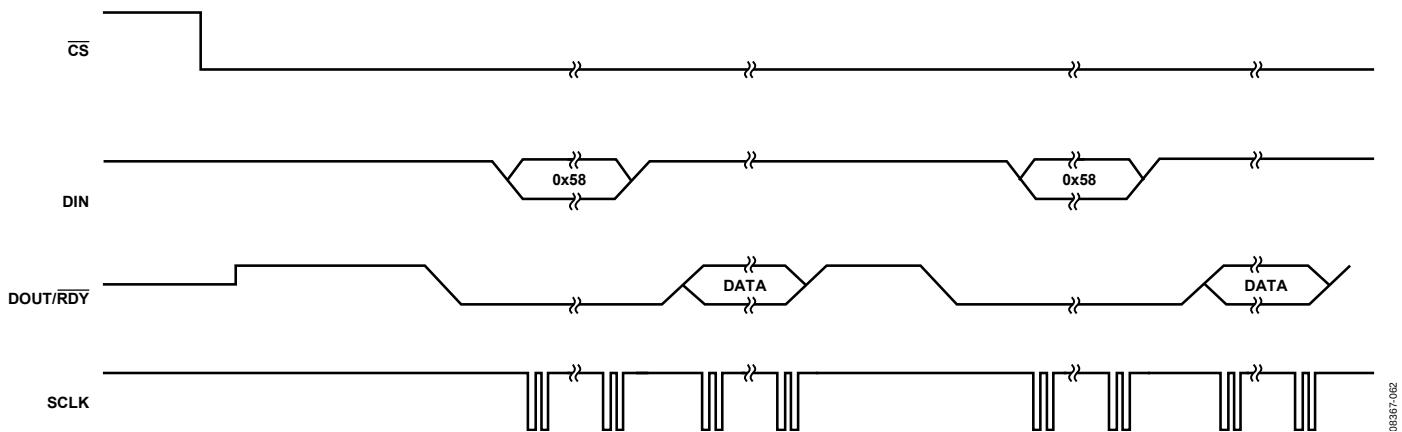
Figure 26. Continuous Conversion
