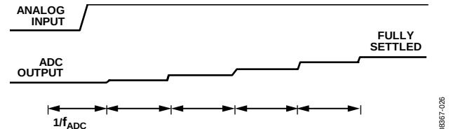
Figure 30. Asynchronous Step Change in Analog Input
