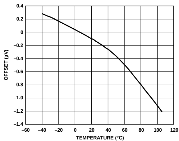
Figure 16. Offset vs. Temperature (Gain = 128, Chop Disabled)
