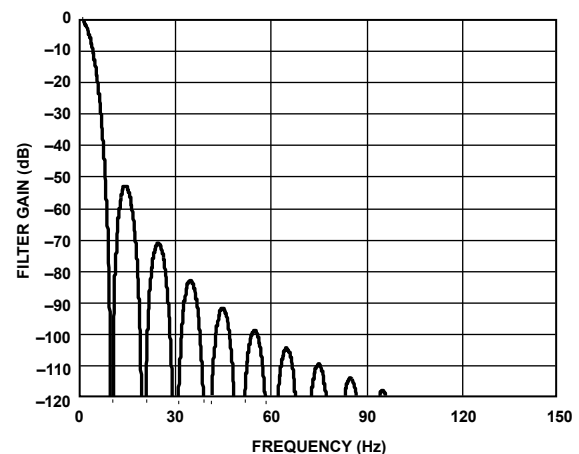
Figure 34. Sinc 4 Filter Response (FS[9:0] = 480)
