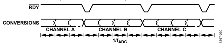
Figure 24. Channel Sequencer
