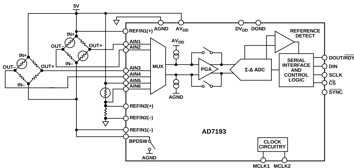
Figure 68. Typical Application (Flowmeter)
