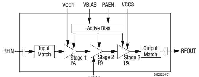
Figure 1. SKY66292-11 Block Diagram
