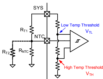
Figure 12: NTC Function Block
