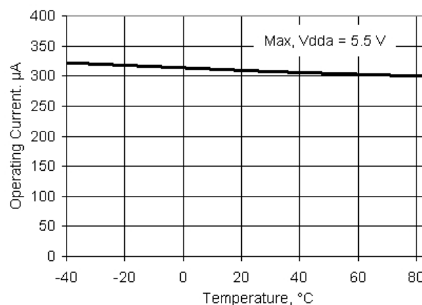
Figure 11-57. VDAC Operating Current vs Temperature, 1 V Mode, High speed mode
