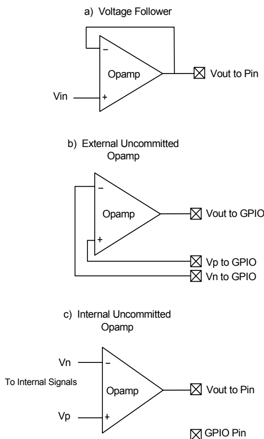
Figure 8-7. Opamp Configurations
