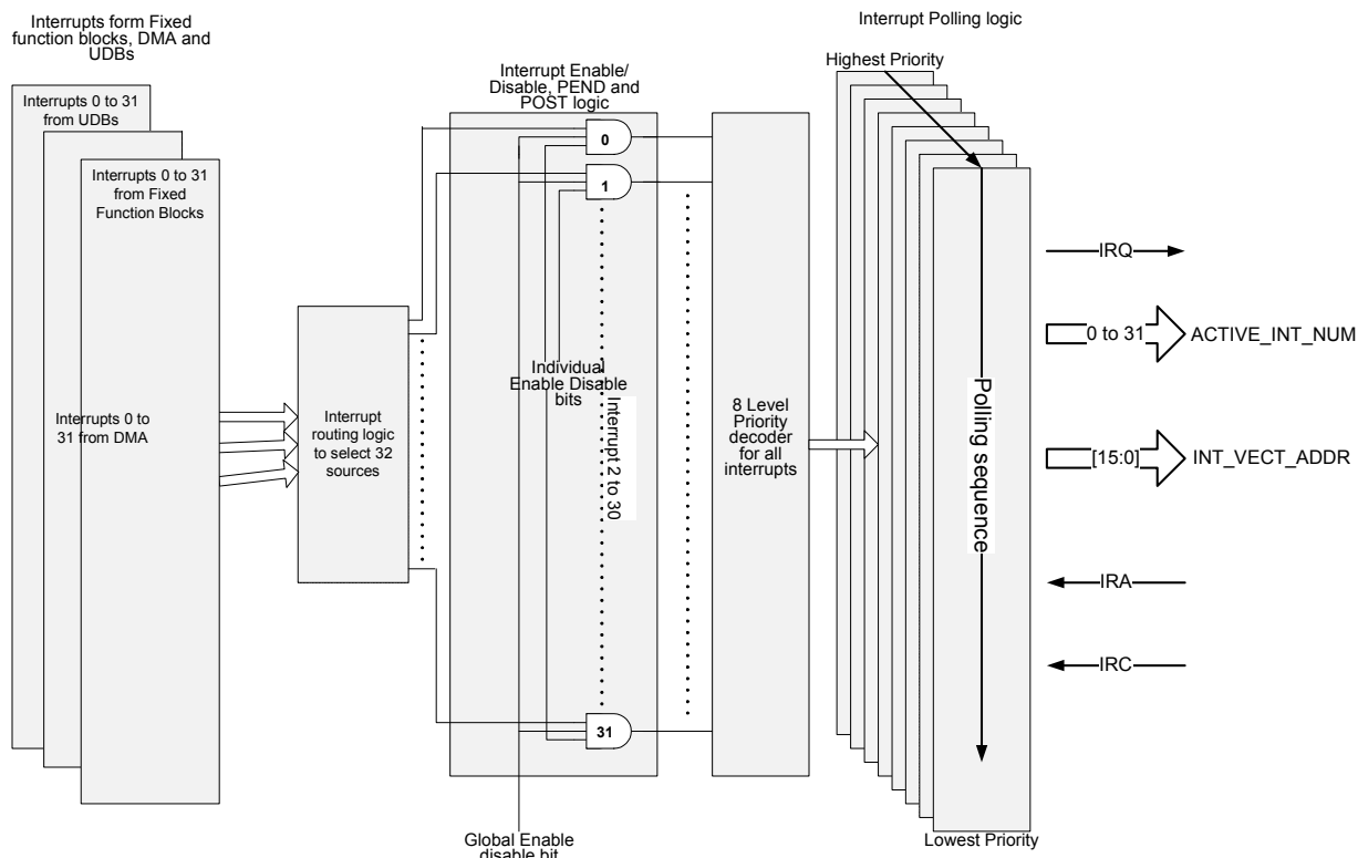
Figure 4-3. Interrupt Structure
