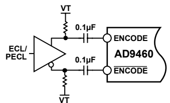
Figure 49. Differential ECL for Encode
