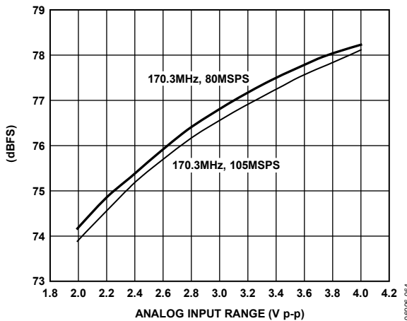
Figure 41. SNR vs. Analog Input Range
