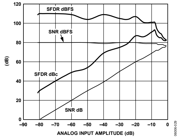
Figure 28. 105 MSPS, 170.3 MHz SNR/SFDR vs. Analog Input Level, CMOS Output Mode
