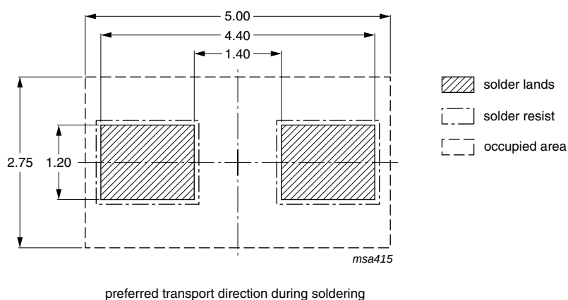
Fig 15. Wave soldering footprint SOD323 (SC-76)
