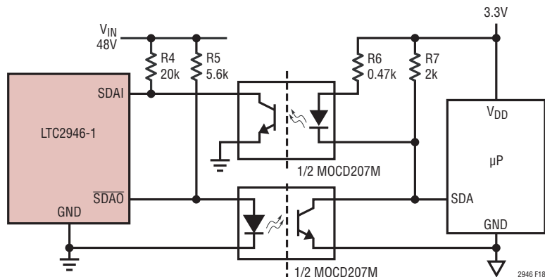
Figure 18. Opto-Isolation of a 1.5kHz I 2 C Interface Between LTC2946-1 and Microcontroller (SCL Omitted for Clarity)
