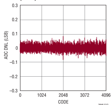
ADC Differential Nonlinearity (ADIN)
