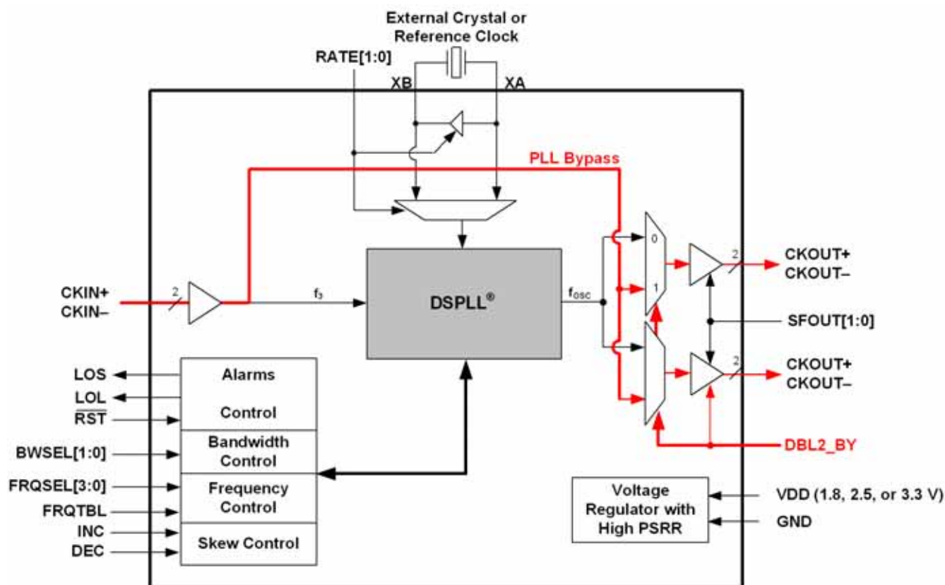
Figure 6. Bypass Signal
