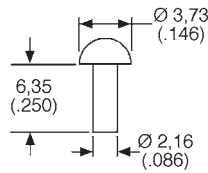
Blanking Plugs for Signal Cavities
