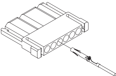
Contact Insertion - Slimline
