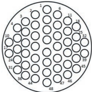
Shell Size 24 0 Power 48 Signal
