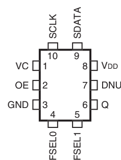
IDT8N0QV01 Rev H 10-lead ceramic 5mm x 7mm x 1.55mm package body CD Package Top View
