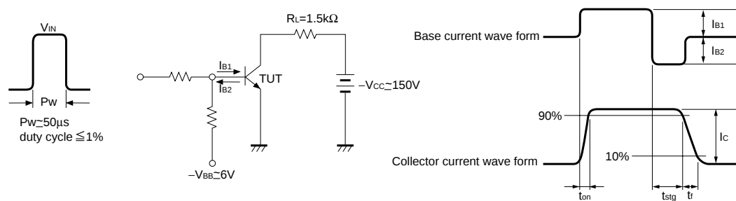
Fig.10 Switching time measurement circuit
