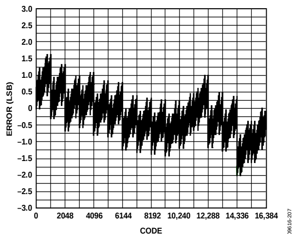
Figure 78. Typical INL, 20 mA at 25°C
