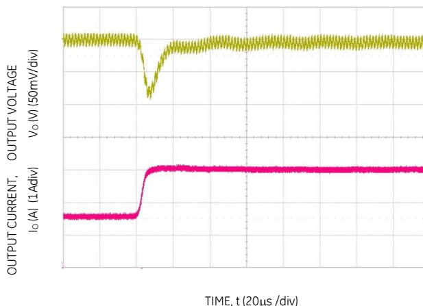
Figure 34. Transient Response to Dynamic Load Change from 50% to 100% at 12Vin, C_{out}=1x47\mu\text{F} , C_{Tune}=820\text{pF} & R_{Tune}=267
