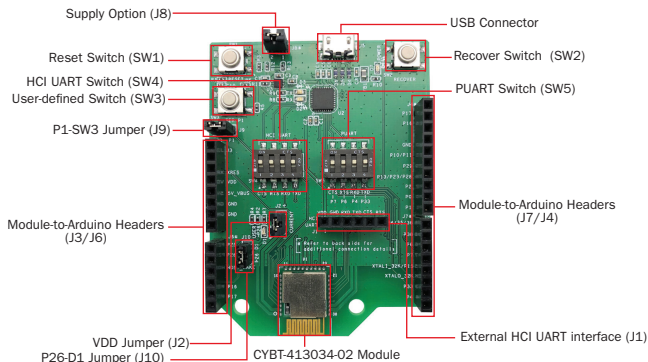
Figure 1: CYBT-413034-EVAL Top View
