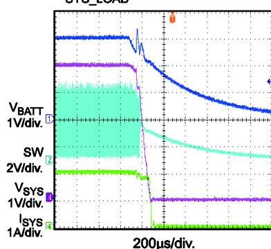
Power Off, Boost Mode V_{SYS\_SET}=5V , V_{BATT}=3V , R_{SYS\_LOAD}=2.5\Omega
