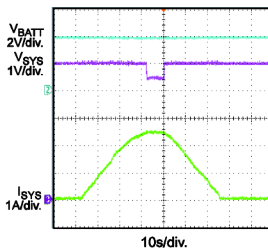
SYS Output Current Limit V_{SYS\_SET}=5V , V_{BATT}=3.7V , I_{OLIM\_SET}=2.5A
