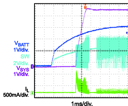
Power On, Boost Mode V_{SYS\_SET}=5V , V_{BATT}=3.7V , No SYS Load
