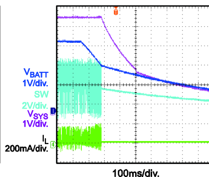
Power Off, Boost Mode V_{SYS\_SET}=5V , V_{BATT}=3.7V , No SYS Load
