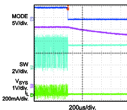
Mode Off, Boost Mode V_{SYS\_SET}=5V , V_{BATT}=3.7V , No SYS Load
