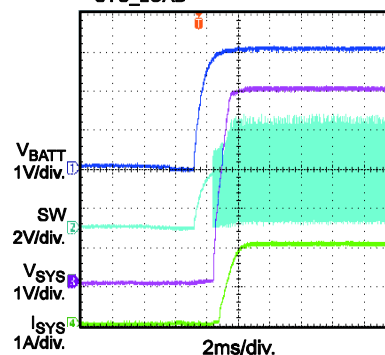
Power On, Boost Mode V_{SYS\_SET}=5V , V_{BATT}=3V , R_{SYS\_LOAD}=2.5\Omega
