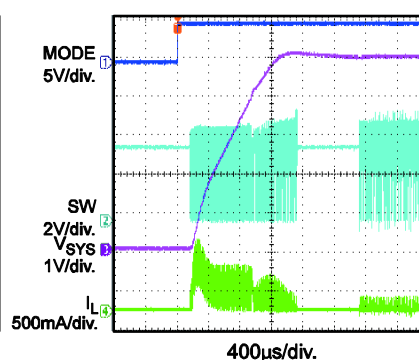
Mode On, Boost Mode V_{SYS\_SET}=5V , V_{BATT}=3.7V , No SYS Load
