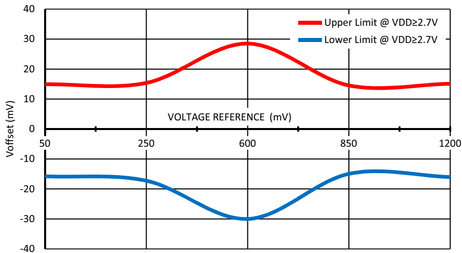
Figure 53. Typical Buffer Input Voltage Offset vs. Voltage Reference at T = (-40.... +85)^{\circ}\text{C} , Buffer Bandwidth = 1 kHz, V_{hys} = 0 mV, Gain = 1.
