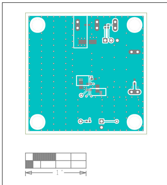
MAXM15466 EV Kit PCB Layout—Top Layer
