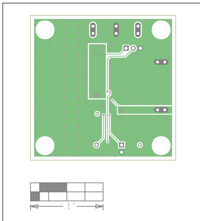
MAXM15466 EV Kit PCB Layout—Layer 3 Power
