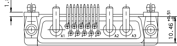
LAYOUT DIMENSIONS (after plating) CONNECTOR SIDE VIEW
