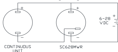
Wiring Diagram
