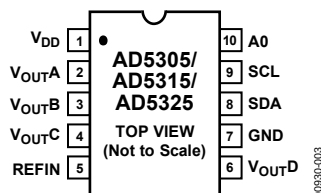
Figure 3. Pin Configuration
