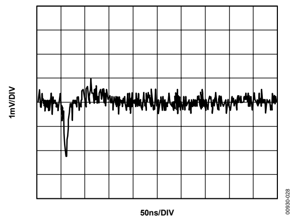
Figure 26. DAC-to-DAC Crosstalk
