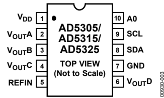
Figure 3. Pin Configuration
