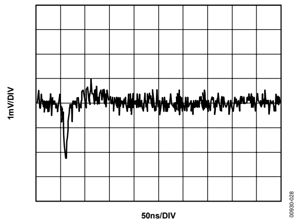
Figure 26. DAC-to-DAC Crosstalk
