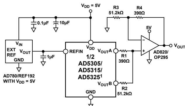
Figure 40. Coarse/Fine Adjustment
