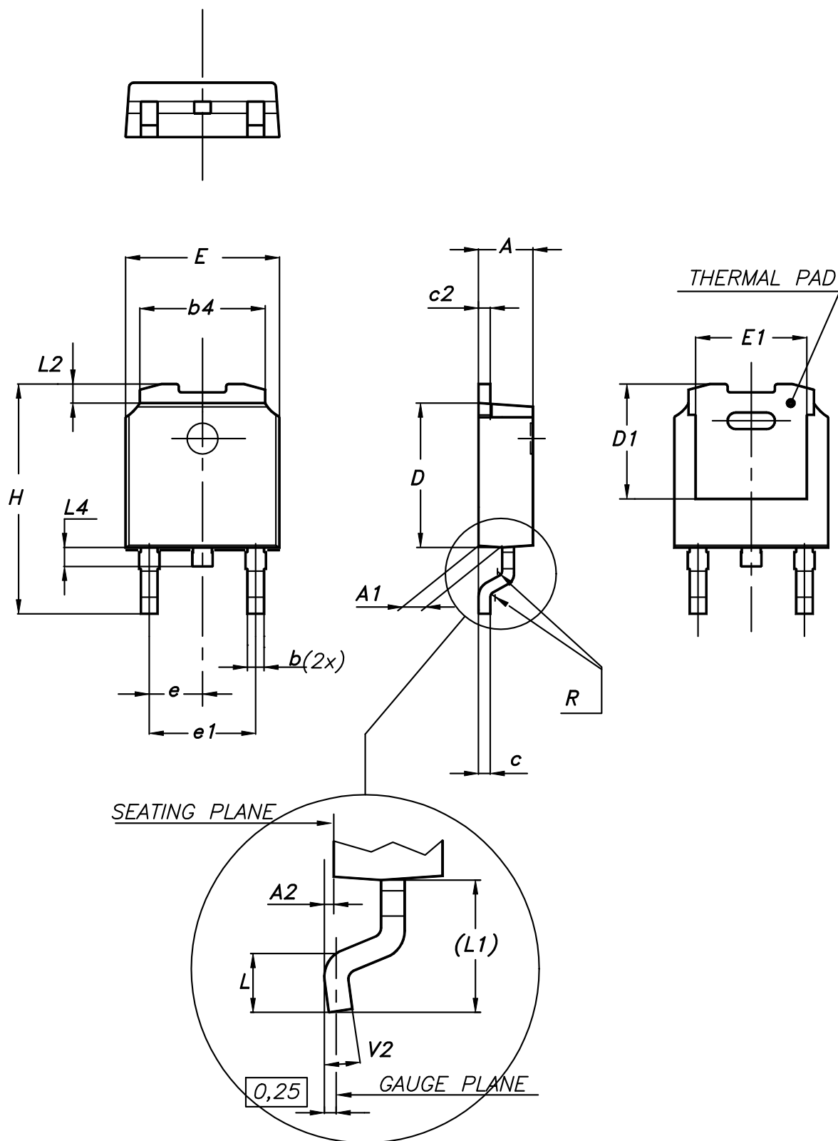
Figure 19. DPAK (TO-252) type A2 package outline
