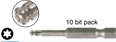
745 Ball End TORX® Bits. 1/4" Hex Drive, Length 2.0"/50mm
